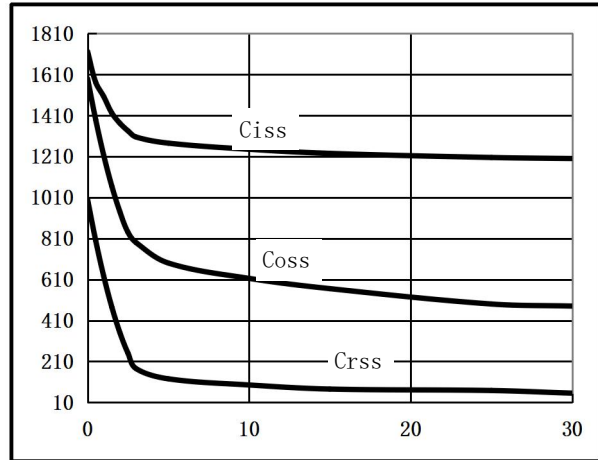
Fig.2 Capacitance Characteristics
